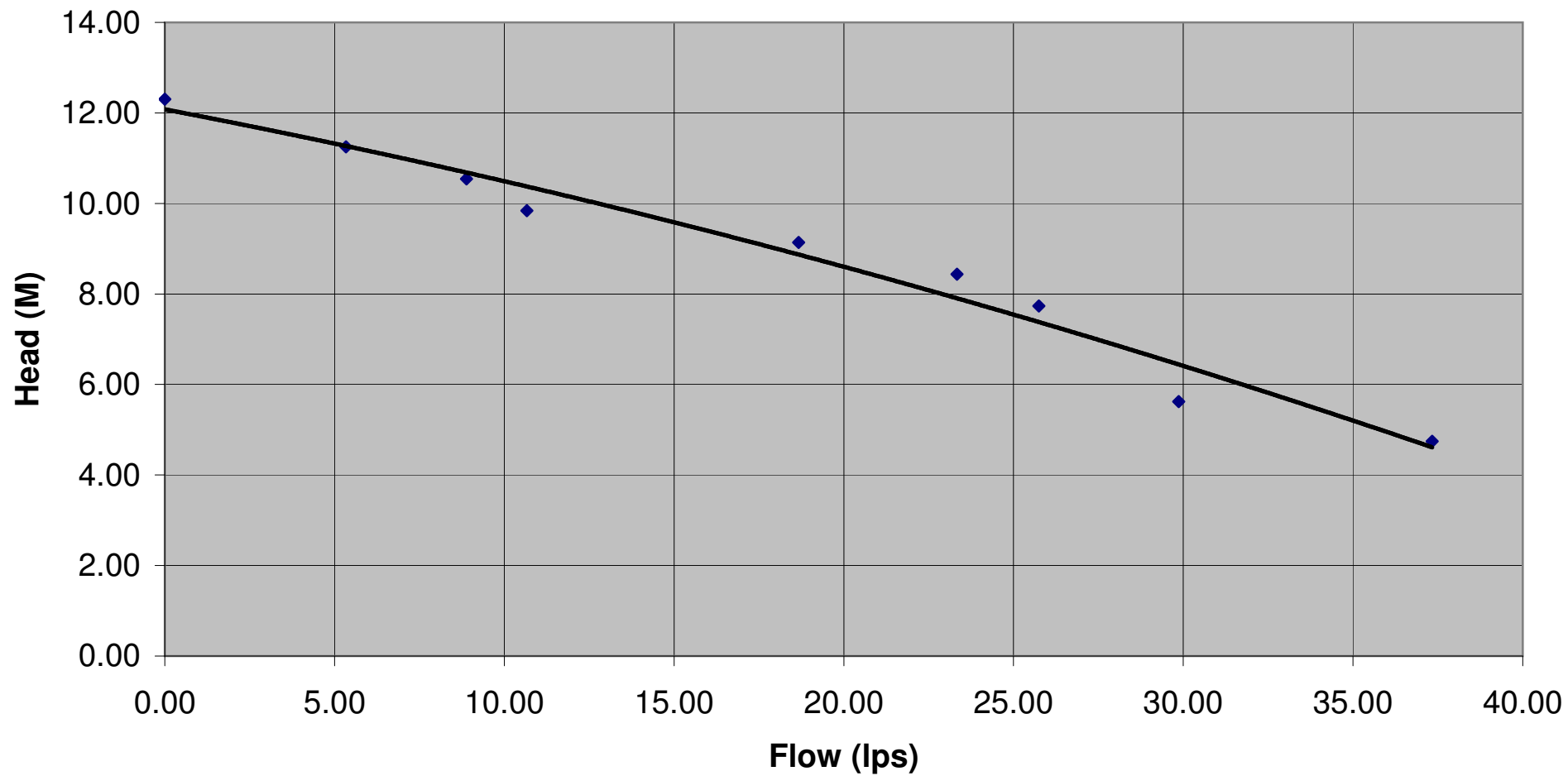
Pump Curve - 402 Macipump (365mm Dia, 40mm Deep, 720 RPM)
